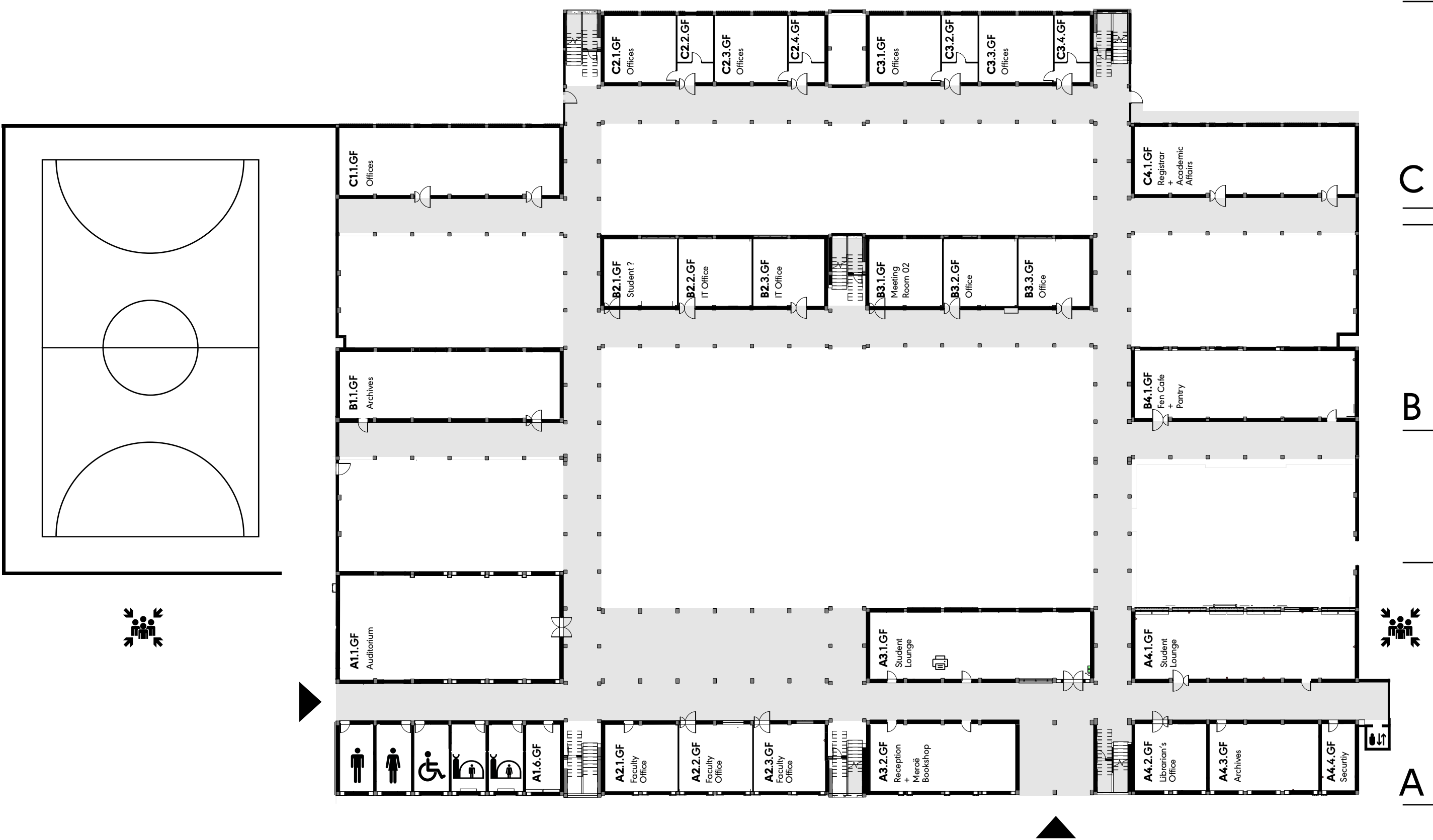
Ground Floor (GF)
